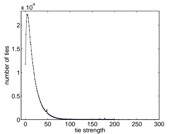
FIG. 1: The distribution of the strength of ties, measured as the number of triads each tie participates in.
