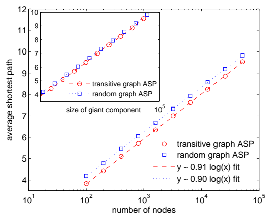
FIG. 7: Numerical comparison of the average shortest path in triangle graphs and Erdős-Renyi graphs with the same number of nodes and edges. The inset shows the average shortest path as a function of the size of the giant component rather than the total number of nodes.
